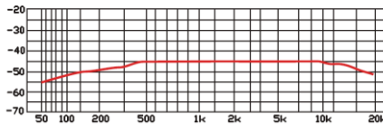
Figure 2: Frequency response
